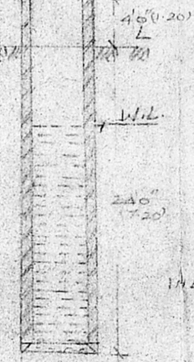
SECTION OF WELL SCALE 1" = 8'0" EX. 4' 2" WELL
